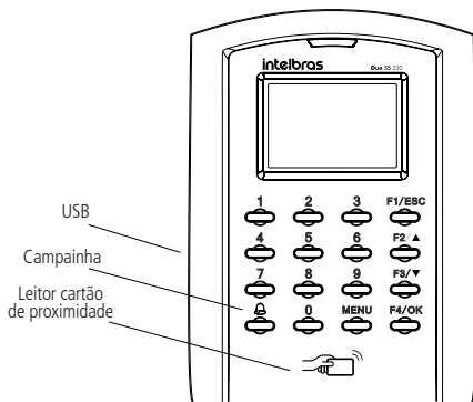
Vista frontal Duo SS 230 / Duo SS 230 MF
