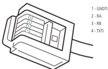
Pinos do conector RJ11
