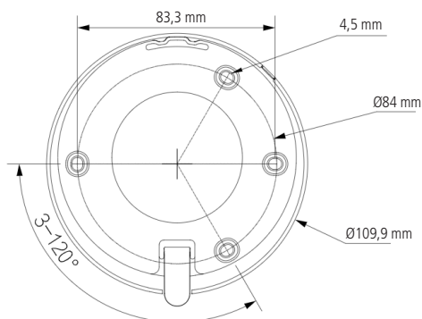
Vista lateral VIPW 1230 D
