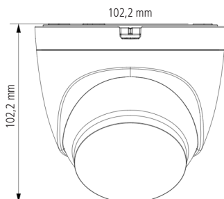
Vista frontal VIPW 1230 D
