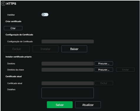
HTTPS
