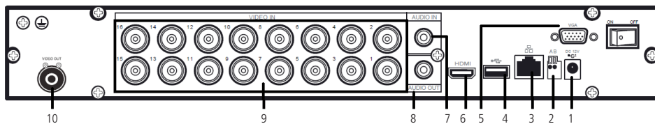
Painel traseiro
